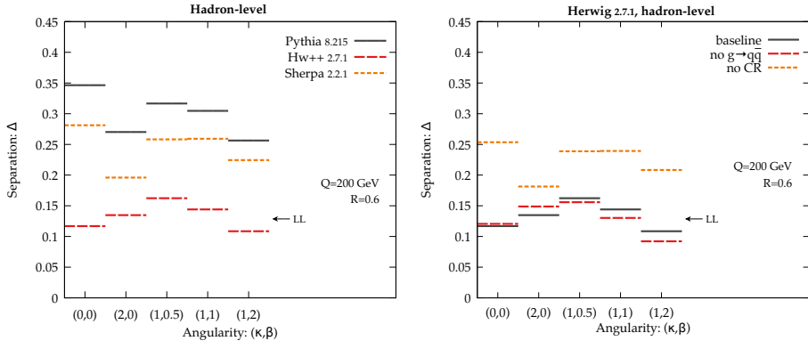
Fig. 1. The classifier separation \Delta for five angularities for an idealized case of e^+e^- collisions. Left panel shows results of various generators. The right panel shows different setting variations for Herwig++ 2.7.1.
