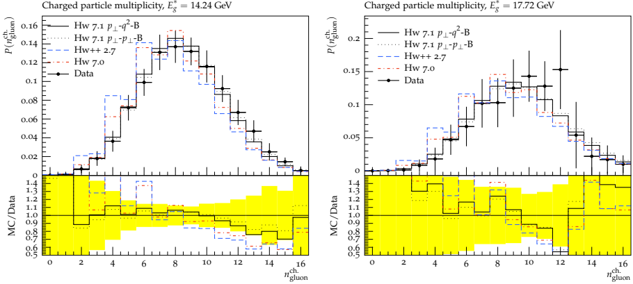
Fig. 2. Multiplicity distribution of charged particles in gluon jets for two different gluon energies compared to data from OPAL [21].
