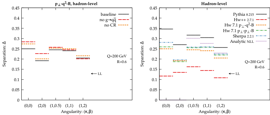
Fig. 3. The classifier separation \Delta for five angularities, determined from various generators for an idealised case of e^+e^- collisions. The first two columns correspond to IRC-unsafe distributions (multiplicity and p_T^D ), while the last three columns are the IRC-safe angularities.
