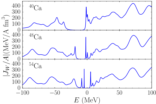
Fig. 2. Volume integral of the imaginary part of the neutron optical potentials, J_W(E) , for the ^{40}\text{Ca} , ^{48}\text{Ca} and ^{54}\text{Ca} targets. Calculated at N_{\max} = 11 .
