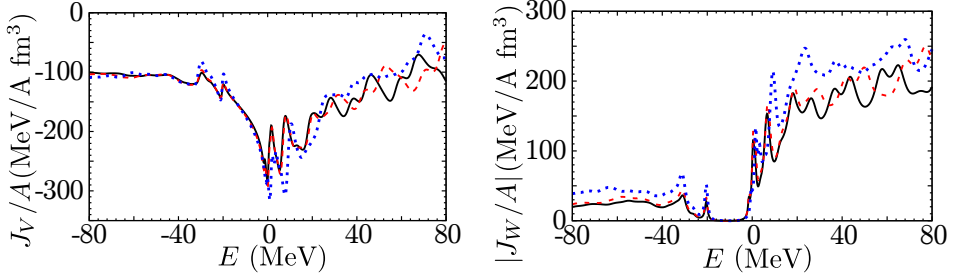
Fig. 1. Volume integrals of the real (left) and imaginary (right) parts of the neutron- ^{16}\text{O} optical potential calculated for different numbers oscillator shells in the model space: N_{\max} = 7 (dotted), 11 (dashed) and 13 (solid lines). Note that \Im m\{\Sigma^*(E = E_F)\} = 0 , so J_W(E = E_F) = 0 , where E_F is the Fermi energy. Thus, the potential for particle (holes) states is above (below) the gap in the J_W plot.
