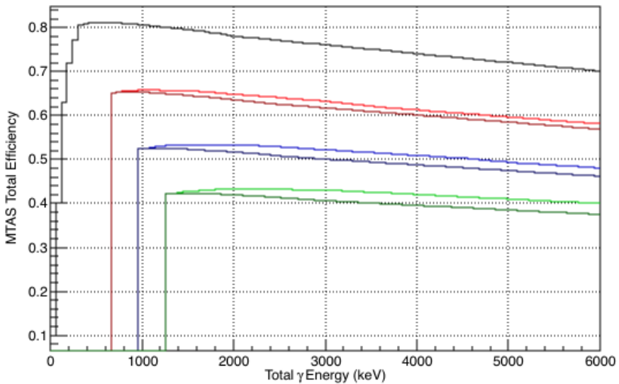
Fig. 3. (Color online) Plot of the range of MTAS (including auxiliary detectors) total efficiencies for 1 \gamma ray (top, black), 2 \gamma rays (second from top, red), 3 \gamma rays (third from top, blue), and 4 \gamma rays (fourth from top, green). The total \gamma energy is the sum of all \gamma rays considered. The range in efficiencies for each number of \gamma rays represents the uncertainty based on not knowing the energies of the individual \gamma rays. The sharp drops at 600, 900, and 1200 keV are due to the 300 keV cut on individual \gamma ray energy in the calculation.
