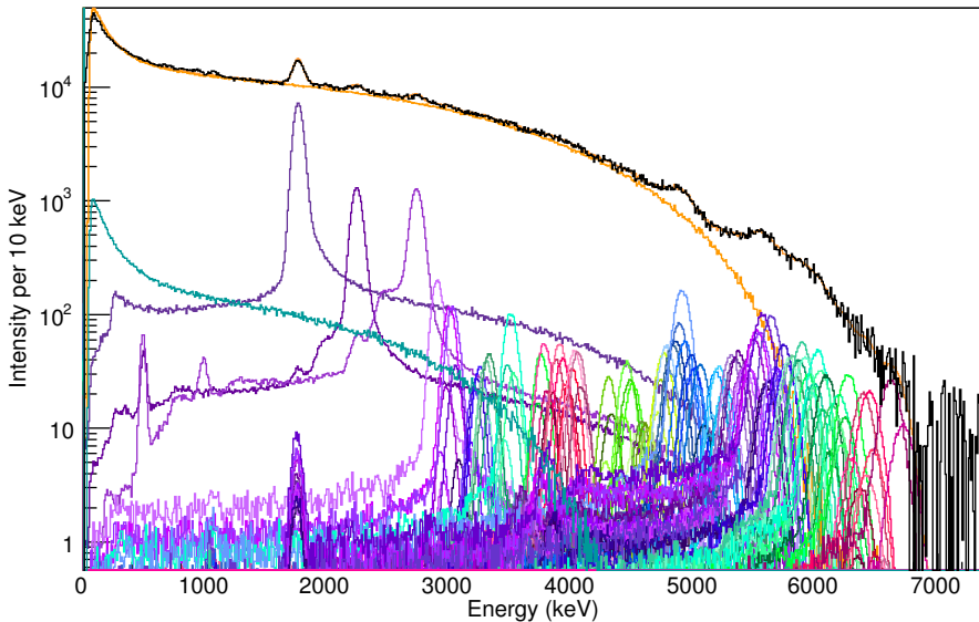
Fig. 1. (Color online) Fit of the individual level decays to the total extracted MTAS data for ^{96\text{gs}}\text{Y} (black). The ground state feeding (orange) and the feeding to the 1581 keV 0^+ excited state (blue-green) are the wide non-peaked distributions that increase at lower energies.
