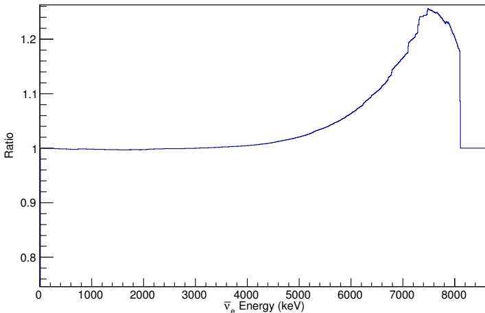
Fig. 4. Ratio of the calculated MTAS data to the 2007 ENSDF data of the \bar{\nu}_e flux as a function of energy for ^{235}\text{U} fuel for ^{92}\text{Rb} . This correction is in the opposite direction to reductions in ground state to ground state feedings based on nuclei affected by the Pandemonium effect.
