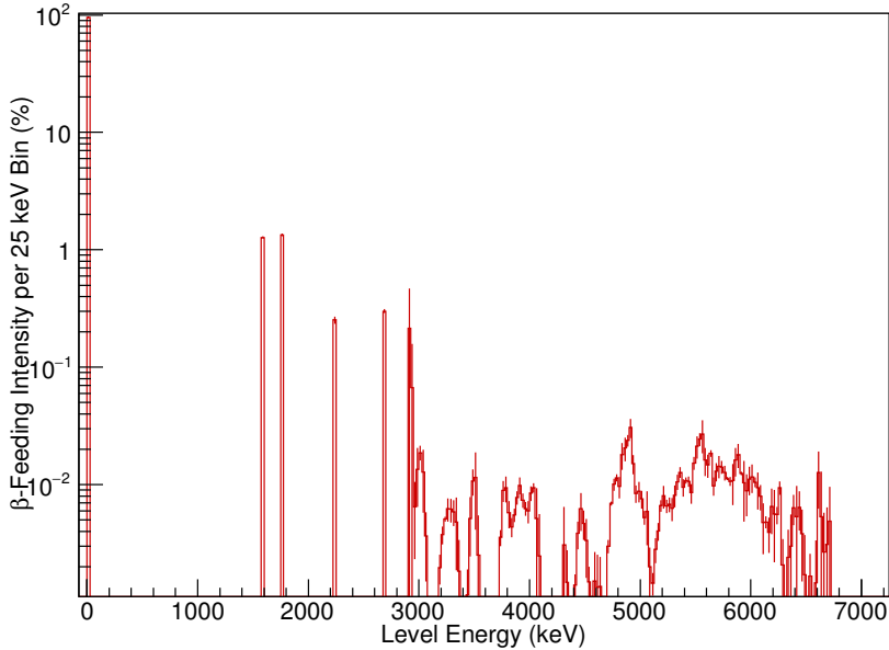
Fig. 2. Calculated \beta -feeding intensities for the ^{96\text{gs}}\text{Y} . Above 6600 keV, the intensities are consistent with zero. The large uncertainty just below 3000 keV comes from varying the end point and this type of effect is described in [10].
