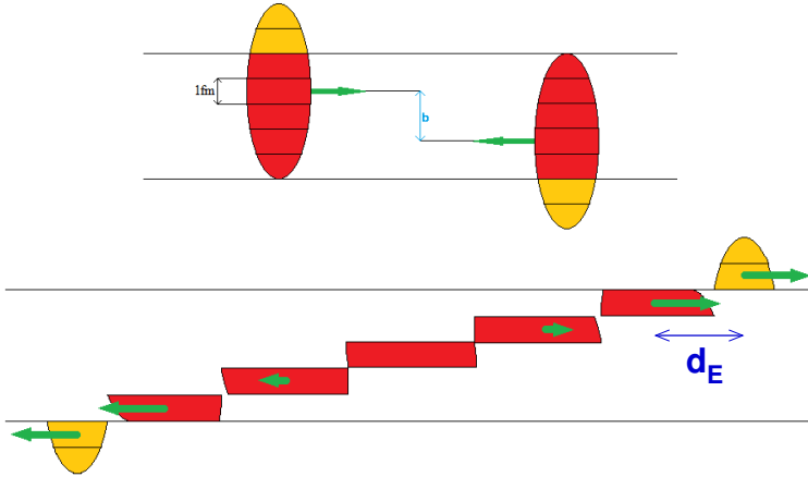
Fig. 7. Sketch of the model of ultrarelativistic heavy-ion collisions proposed in Ref. [15] before the collision (top) and after the collision (bottom). d_E illustrates the correspondence between this model and spectator-induced electromagnetic effects in charged pion emission, which were its original motivation (see Fig. 4).
