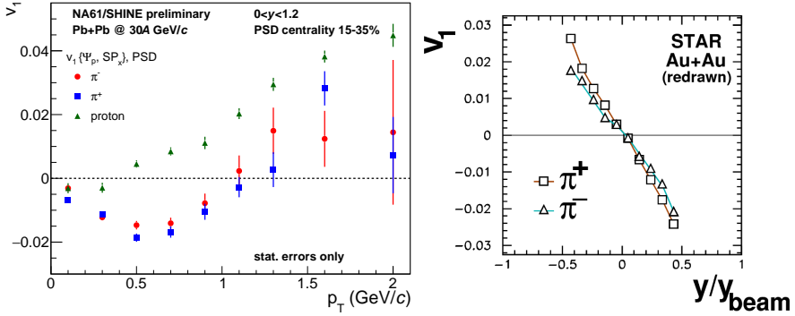
Fig. 5. Directed flow of charged pions and protons as a function of transverse momentum for 15% to 35% centrality class of Pb+Pb collisions at 30A GeV/c beam momentum [12] (left) possibly showing charge splitting of the flow for pions, sensitive to spectator-induced electromagnetic effects, first observed in Au+Au collisions at \sqrt{s_{NN}} = 7.7 GeV [13] (right; original data from Ref. [6]). Only statistical uncertainties are shown.
