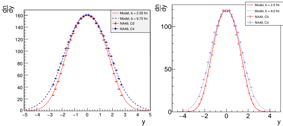
Fig. 8. Change of width of the \pi^- rapidity distribution from peripheral to central Pb+Pb collisions described by the fire streaks model for collisions at 158A GeV/ c beam momentum (left; plot from Ref. [15]) and at 40A GeV/ c beam momentum (right; plot from Ref. [18]). In both cases, experimental data come from Ref. [19] and are scaled to the same peak height so that visual shape comparison is feasible.
