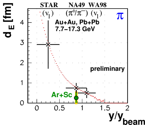
Fig. 4. Dependence of the distance d_E between pion emission point and the spectator system on pion rapidity. Au+Au and Pb+Pb points come from analysis of experimental data from Refs. [6, 10, 11]. The new NA61/SHINE Ar+Sc point [9] corresponds to optimal description of \pi^+/\pi^- ratio in the intermediate centrality Ar+Sc collisions.
