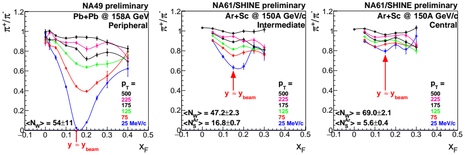
Fig. 1. New NA61/SHINE results [9] on the \pi^+/\pi^- ratio at the top CERN SPS beam momentum as a function of x_F for several values of transverse momentum, in intermediate centrality Ar+Sc and central Ar+Sc collisions (middle and right) compared to peripheral Pb+Pb collisions [8] (left). Only statistical uncertainties are shown.
