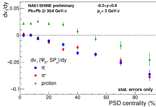
Fig. 6. Slope of directed flow at midrapidity for charged pions and protons as a function of centrality estimated with energy deposited in PSD calorimeter in Pb+Pb collisions at 30A GeV/c beam momentum. Only statistical uncertainties are shown.
