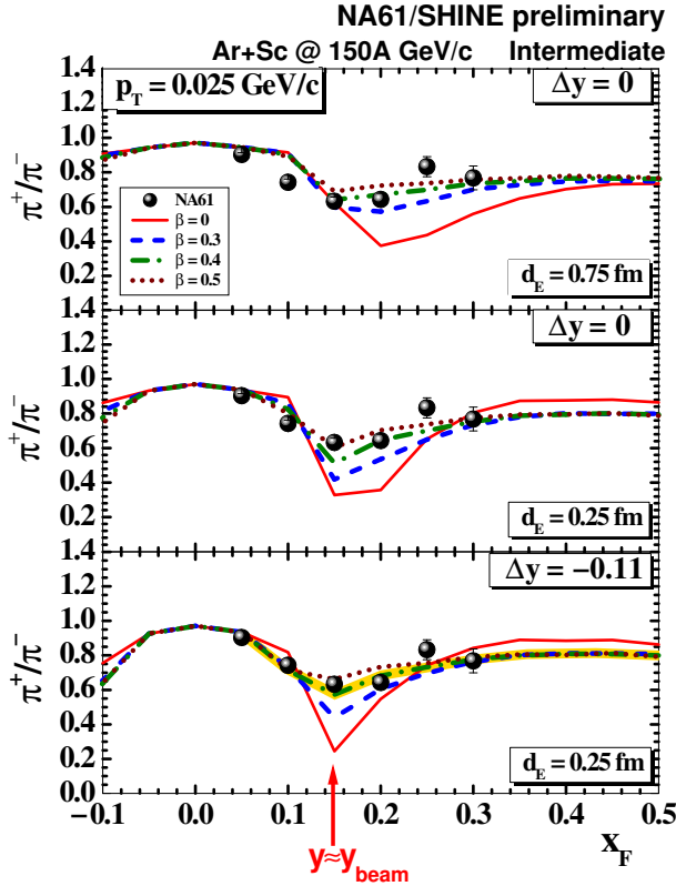
Fig. 3. (Colour on-line) ‘Fitting’ of the improved model [9] of spectator-induced electromagnetic effects in ultrarelativistic nuclear collisions to the lowest p_T (the largest EM effect) results on the \pi^+/\pi^- ratio in the intermediate centrality Ar+Sc collisions (lowest lying points in the middle plot in Fig. 1). Different lines represent different values of the \beta parameter, top panel differs in d_E from two others, while the bottom panel differs in \Delta y from the top and the middle. The model calculation associated with combination of parameters judged to be optimal is highlighted with thick light grey/yellow line in the bottom panel.
