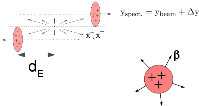
Fig. 2. Sketch of improvements (see the text) to the original model [3] of spectator-induced electromagnetic effects in ultrarelativistic nuclear collisions.
