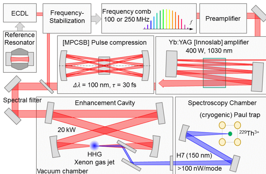
Fig. 6. Schematic outline of the VUV frequency-comb-based laser designed to drive the nuclear clock transition in ^{229\text{m}}\text{Th} .
