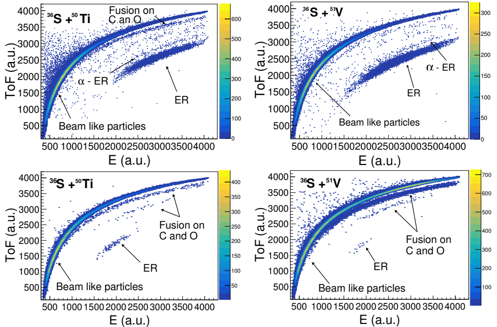
Fig. 1. Time of flight \text{TOF}_3 versus residual energy of the ^{36}\text{S}+^{50}\text{Ti} (on the left) and ^{36}\text{S}+^{51}\text{V} (on the right) systems. The measurements were performed at the incident energies of 100 MeV (at the top) and 78 MeV (at the bottom).
