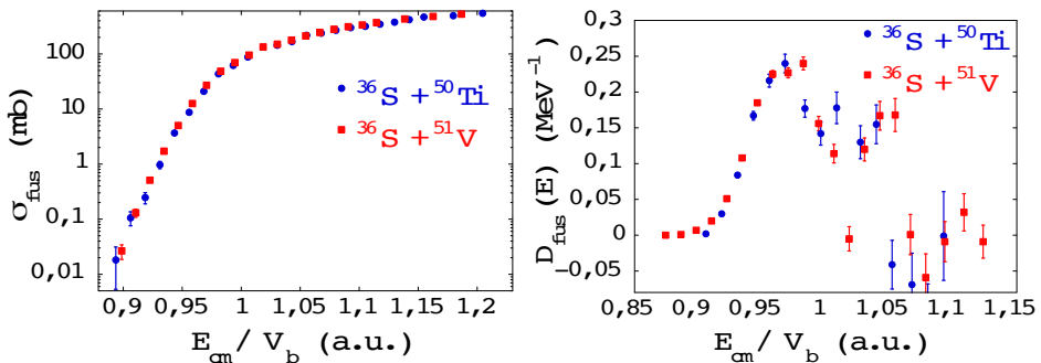
Fig. 2. Comparison of the excitation functions (on the left) and barrier distributions (on the right) for the two fusion reactions. The energy scale is normalized to the height of the two Coulomb barriers.
