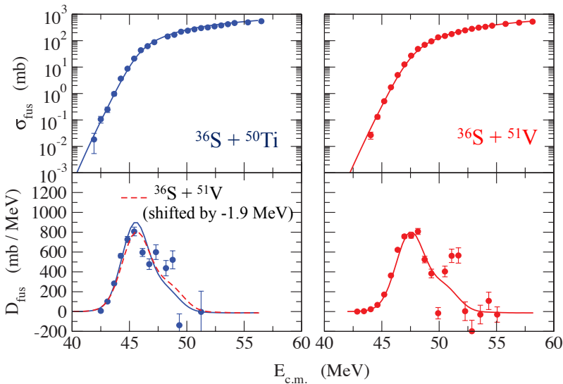
Fig. 3. Excitation functions (top) and fusion barrier distributions (bottom) of ^{36}\text{S}+^{50}\text{Ti} (on the left) and ^{36}\text{S}+^{51}\text{V} (on the right), compared with the CC calculations.
