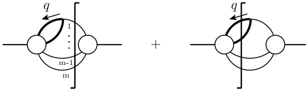
Fig. 1. Cancellation of NLO final-state IR singularities in FDR.
