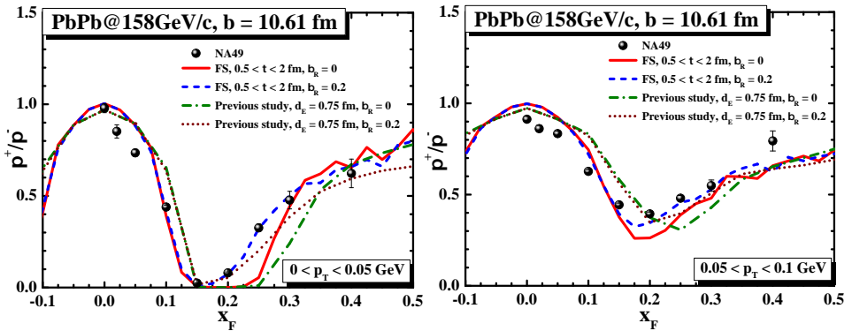
Fig. 4. (Colour on-line) ‘Fitting’ of the fire-streaks-based model [12] (‘FS’) of spectator-induced electromagnetic effects in ultrarelativistic nuclear collisions to the two lowest p_T (the largest EM distortions) results on the \pi^+/\pi^- ratio in the peripheral Pb+Pb collisions [3]. It is compared to calculations within the model (‘Previous study’) used in Sec. 3 to describe Ar+Sc collisions. The model calculation judged to be optimal is the one depicted with dashed blue line (see legends for the parameters).
