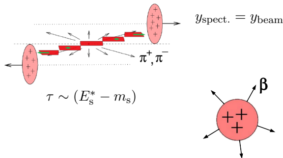
Fig. 3. Sketch of the model of spectator-induced electromagnetic effects built on top of the fire streaks model [11], used to improve description of Pb+Pb collisions, taking into account spectator expansion [12].
