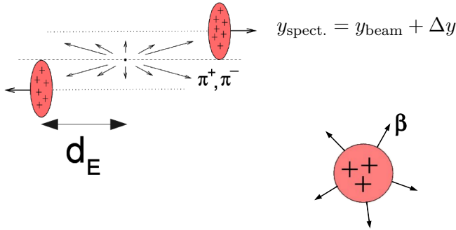
Fig. 1. Sketch of the model of spectator-induced electromagnetic effects used to describe Ar+Sc collisions, taking into account spectator expansion and possible net positive participant charge close to the spectator system [5, 6], based on the original model of [4] initially used for Pb+Pb collisions.
