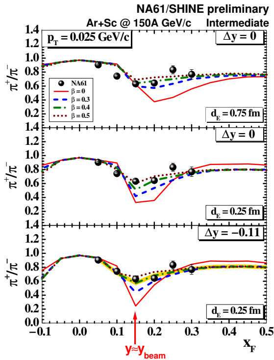
Fig. 2. (Colour on-line) ‘Fitting’ of the improved model [5] of spectator-induced electromagnetic effects in ultrarelativistic nuclear collisions to the lowest p_T (the largest EM effect) results on the \pi^+/\pi^- ratio in the intermediate centrality Ar+Sc collisions. Figure taken from [6]. The model calculation judged to be optimal is the one highlighted with thick light grey/yellow line in the bottom panel (see legends and the text for the parameters).
