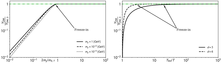
Fig. 1. A typical evolution of the DM yield for the forbidden freeze-in via renormalizable (left) and non-renormalizable (right) operators.
