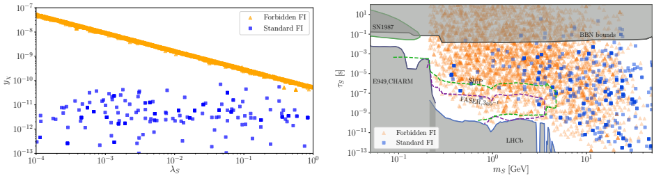
Fig. 3. The parameter space in the \lambda_S – y_\chi plane (left) and the (vacuum) mass versus life-time of S (right).
