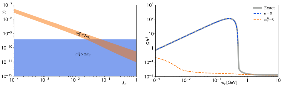
Fig. 2. (Colour on-line) The parameter space in the \lambda_S - y_\chi plane (left) and the dependence of \Omega h^2 on m_\chi (right) given by the numerical solution of the BE (1), assuming thermal mass for S .
