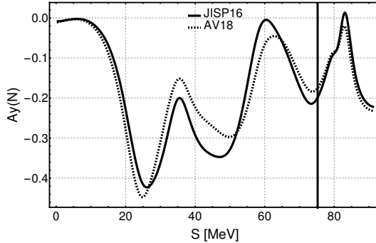
Fig. 2. The comparison of the nucleon analysing power, predicted by JISP16 (solid line) and AV18 (dashed line) models for the deuteron breakup reaction at E_i = 65 MeV, \theta_1 = 74^\circ , \theta_2 = 34^\circ and \varphi_{12} = 178^\circ . The relative difference \Delta at S = 75 MeV (marked with a vertical line) is -0.12 .
