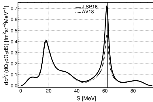
Fig. 1. The comparison of cross sections, predicted by JISP16 (solid line) and AV18 (dashed line) models, for the deuteron breakup reaction at E_i = 65 MeV, \theta_1 = 42^\circ, \theta_2 = 66^\circ and \varphi_{12} = 178^\circ . The relative difference \Delta at S = 62 MeV (marked with a vertical line) is 0.44.
