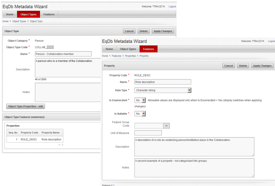
Fig. 4. Exemplary EqDb Metadata Wizard screenshots.
