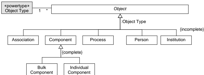
Fig. 1. EqDb objects structure: powertype, supertype and subtypes.
