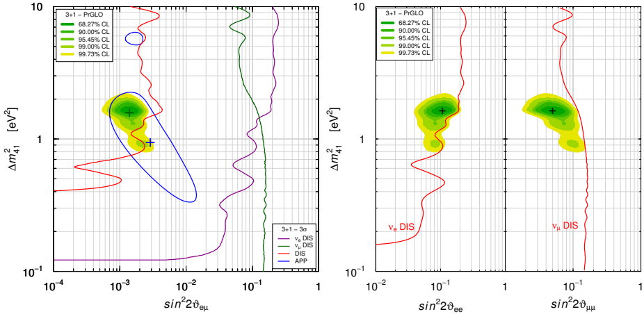
Fig. 1. Allowed regions in the \sin^2 2\vartheta_{e\mu} - \Delta m_{41}^2 , \sin^2 2\vartheta_{ee} - \Delta m_{41}^2 and \sin^2 2\vartheta_{\mu\mu} - \Delta m_{41}^2 planes obtained in the pragmatic 3 + 1 global fit PrGLO of short-baseline neutrino oscillation data compared with the 3\sigma allowed regions obtained from \bar{\nu}_\mu \rightarrow \bar{\nu}_e short-baseline appearance data (APP) and the 3\sigma constraints obtained from \bar{\nu}_e short-baseline disappearance data ( \nu_e DIS), \bar{\nu}_\mu short-baseline disappearance data ( \nu_\mu DIS) and the combined short-baseline disappearance data (DIS). The best-fit points of the global (PrGLO) and APP fits are indicated by crosses.
